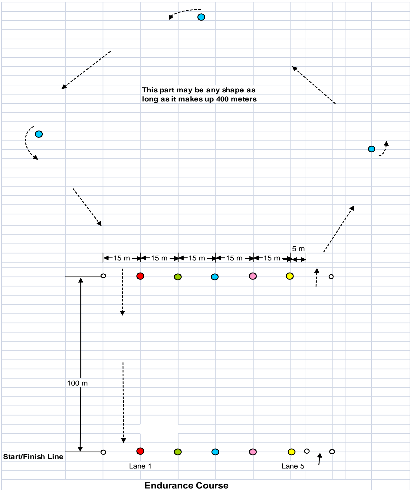
Figure 11.2 –Endurance Race Course Layout (Example Layout)
